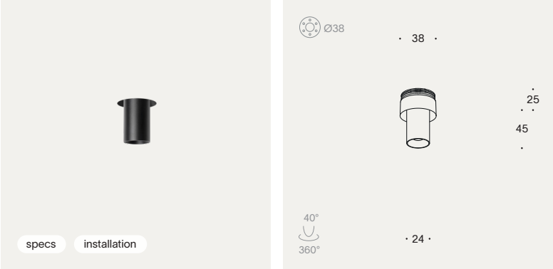
acrobat micro | short
