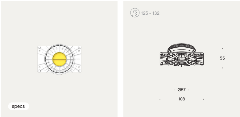
adjustable plaster ring Ø57
