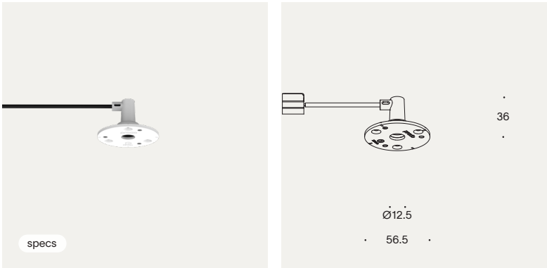
clt ring jack
